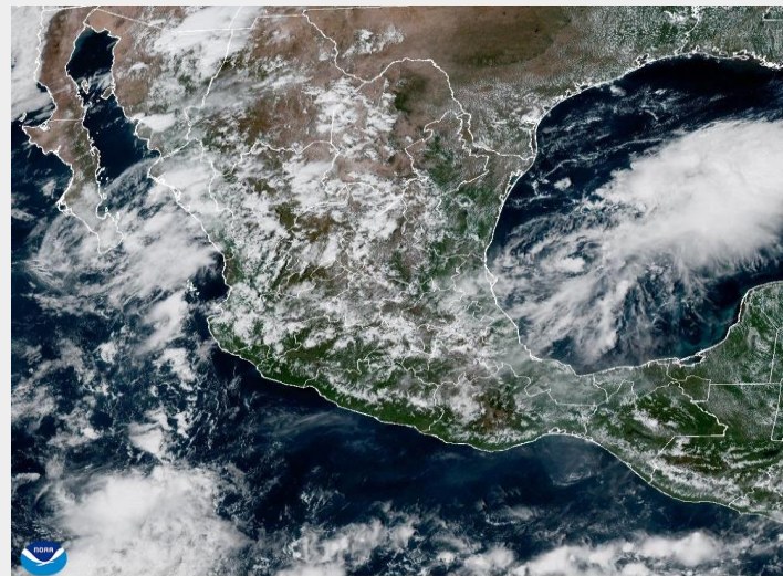
26 Sep 2025 19:10Z - NOAA/NESDIS/STAR - GOES-19 - GEOCOLOR Composite - MEX
