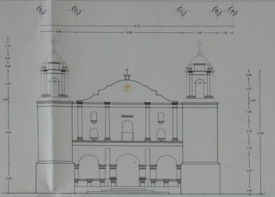
FACHADA PRINCIPAL
